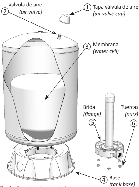
Fig. 8 - Exposed view Fig. 8 - Exposed view
